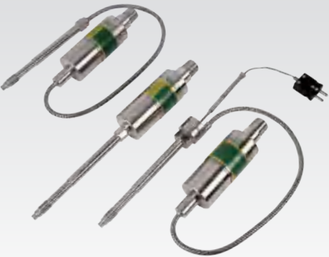
PT110FB Rigid Stem PT120FB Rigid+Flexible Stem PT130FB with Thermocouple
