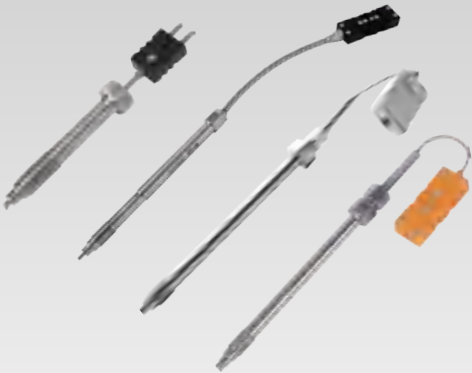
E type K Type J Type Pt100
