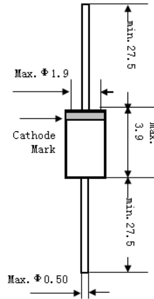
Gass case DO-35 Dimensions in mm
