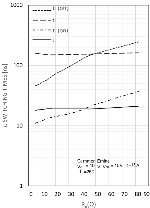
Fig. 7 Switching times vs. gate resistor
