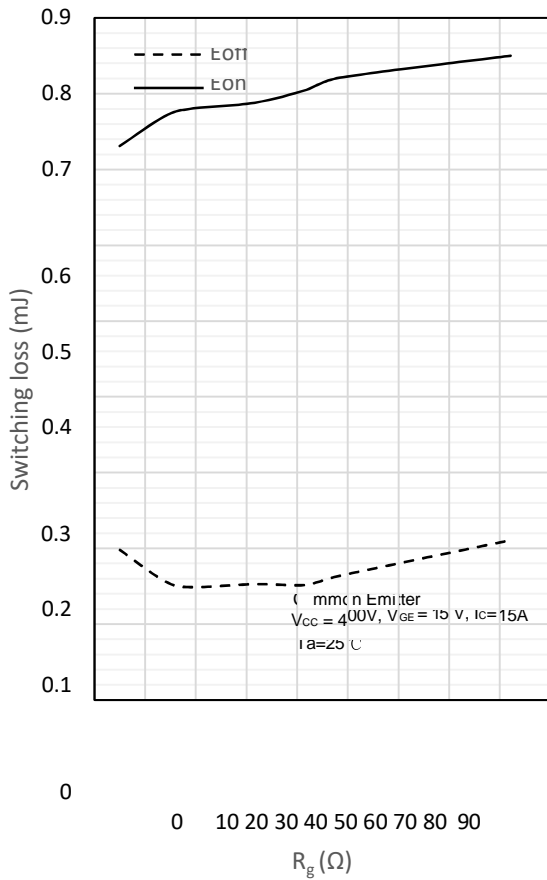
Fig. 9 Switching loss vs. gate resistor
