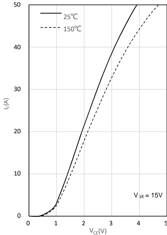
Fig. 6 Saturation voltage characteristics
