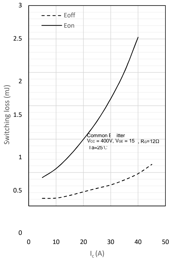
Fig. 10 Switching loss vs. collector current
