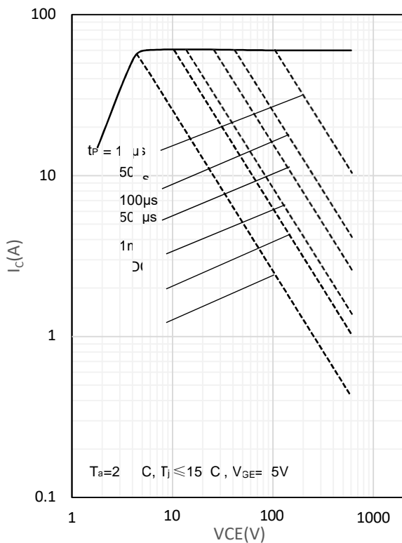
Fig. 1 FBSOA characteristics for TO-220F
