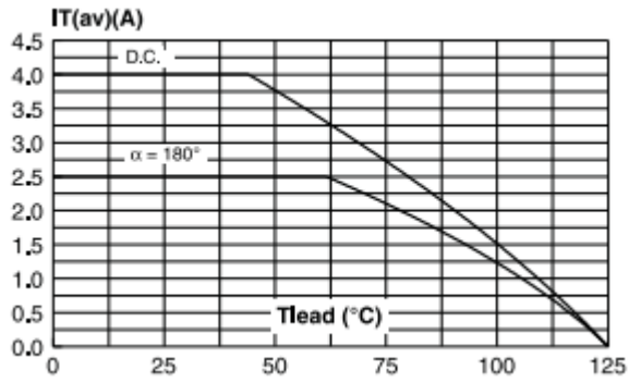
FIG.2: Average on-state current versus lead temperature
