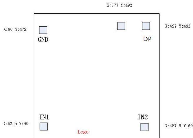
Figure 1-2 FM11NT021TT Bumping Pin Description
