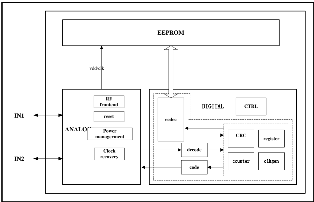
Figure 1-1 FM11NT021TT Block diagram
