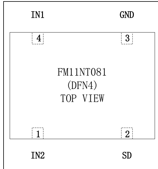
Figure 1-3 DFN4 Pin Description
