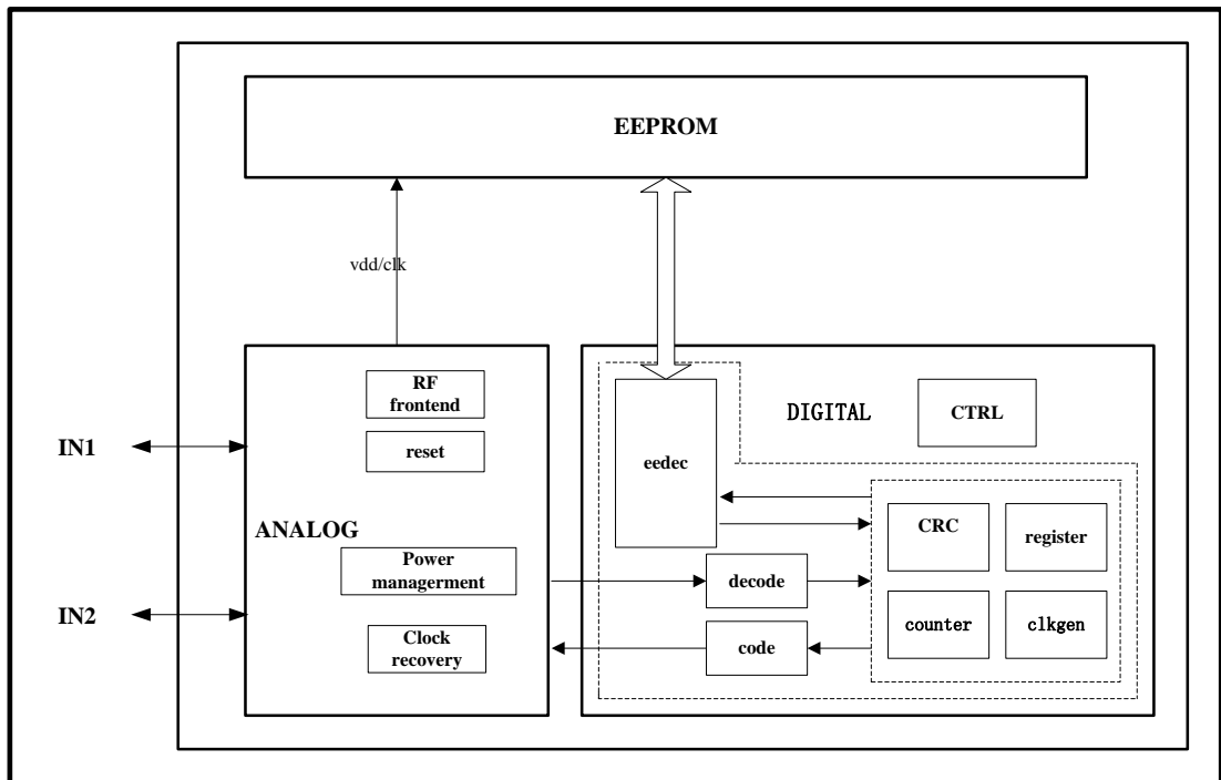
Figure 1-1 FM11NT041 Block diagram
