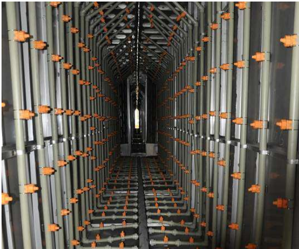
Spraying tunnel
