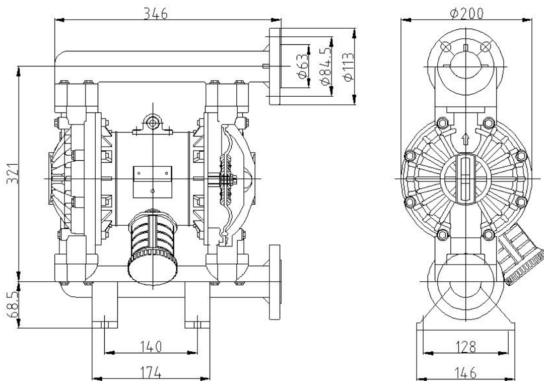
RV25 PVDF (FLANGE)
